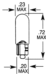
T-1.75 WEDGE BASE
