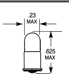
T-1.75 MIDGET FLANGED BASE
