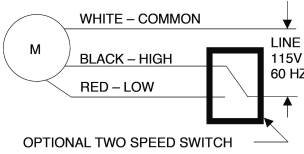
WIRING DIAGRAM
