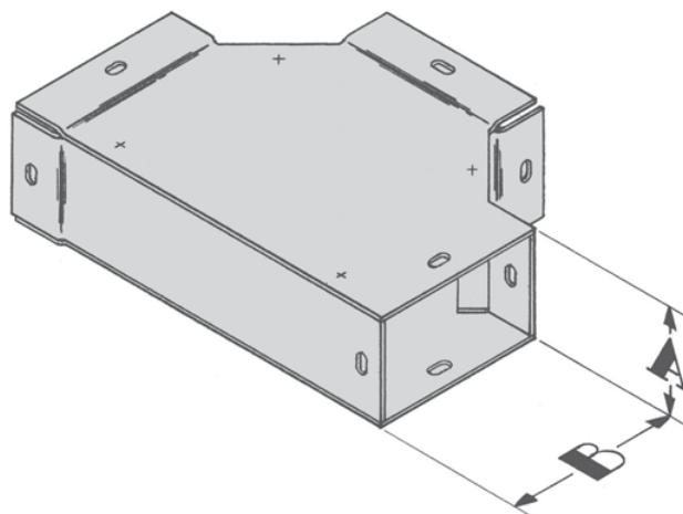
FLAT 90° SHOWN, i.e. TEE-254
