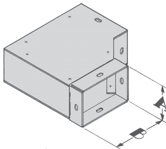
FLAT 90° SHOWN, i.e. L90-254120
