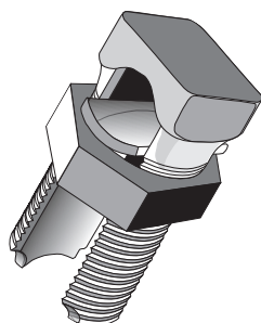
SPLIT-BOLT CONNECTOR
